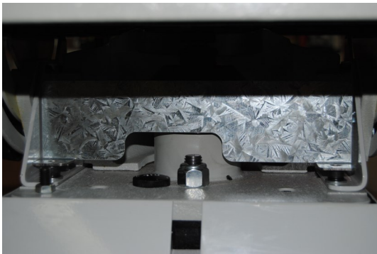
Under table guard to avoid pinch point
